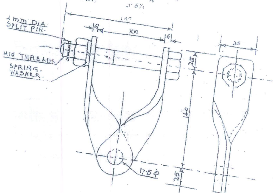
CROSS-ARM STRAPS
